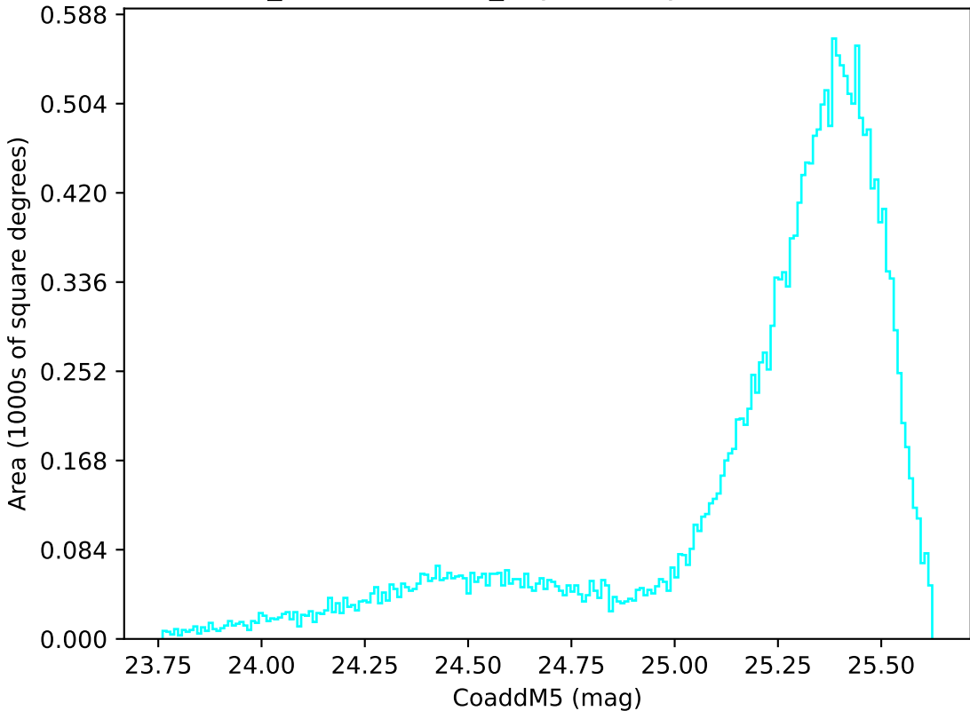
weather_cloudso16v3.4_10yrs All sky u band: CoaddM5
