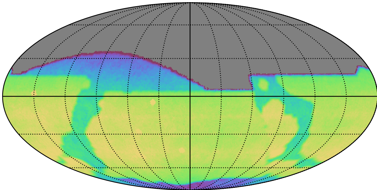
weather_cloudso16v3.4_10yrs All sky r band: CoaddM5
