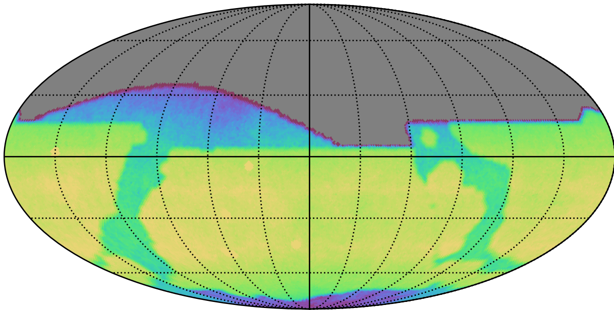
weather_cloudso16v3.4_10yrs All sky i band: CoaddM5
