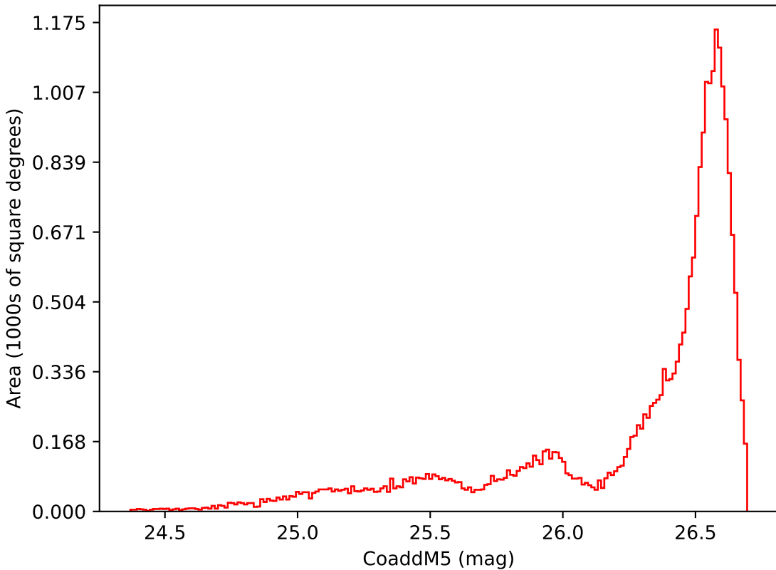
weather_cloudso16v3.4_10yrs All sky i band: CoaddM5
