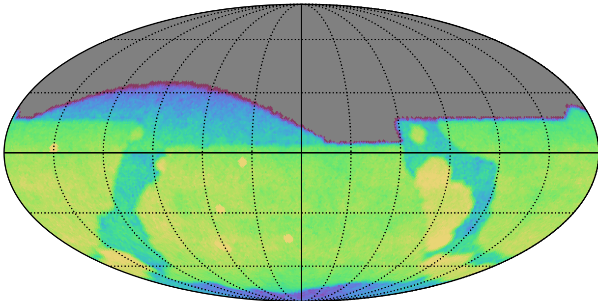
weather_cloudso16v3.4_10yrs All sky g band: CoaddM5
