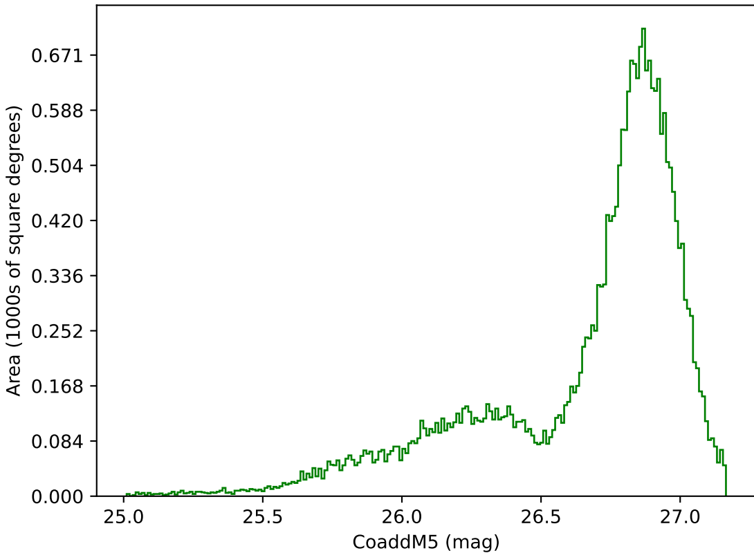
weather_cloudso16v3.4_10yrs All sky g band: CoaddM5
