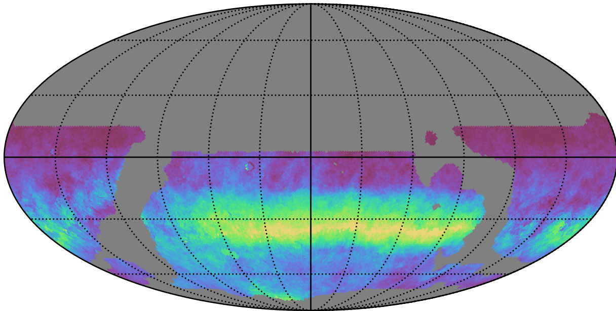
weather_cloudso16v3.4_10yrs WFD r band: AngleRms rotSkyPos
