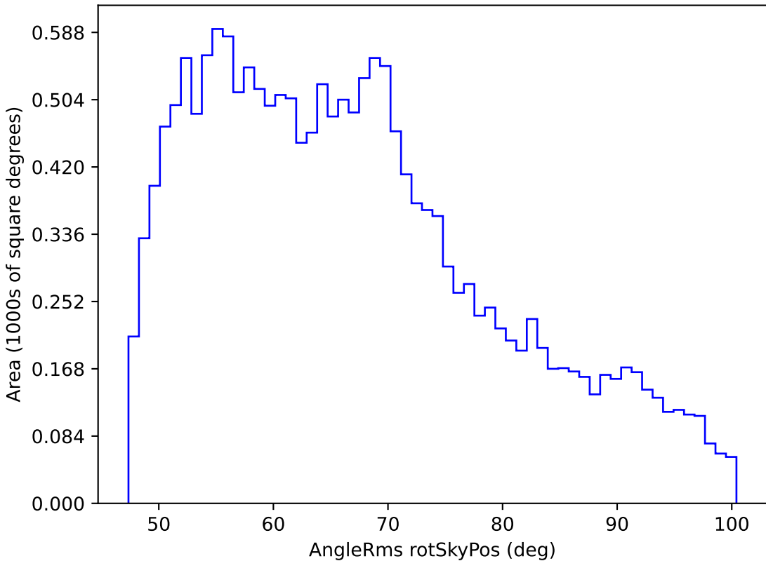
weather_cloudso16v3.4_10yrs WFD r band: AngleRms rotSkyPos
