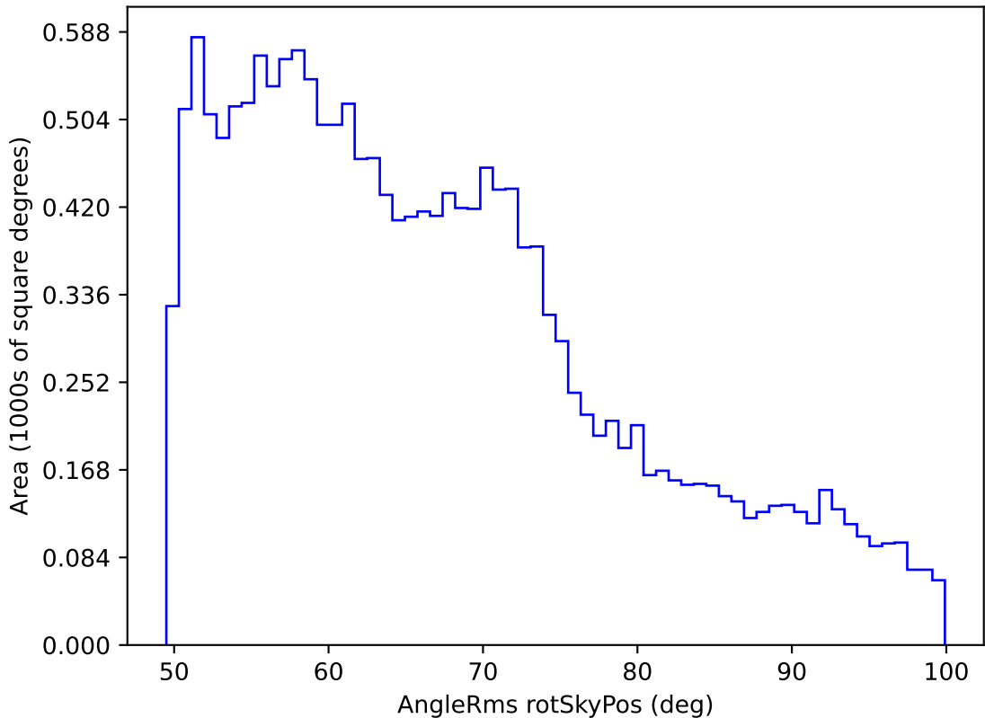
weather_cloudso16v3.4_10yrs WFD all bands: AngleRms rotSkyPos
