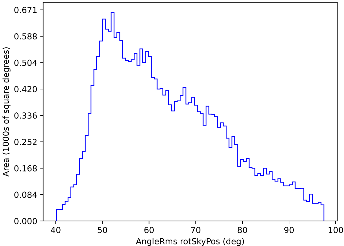
weather_cloudso16v3.4_10yrs All sky z band: AngleRms rotSkyPos
