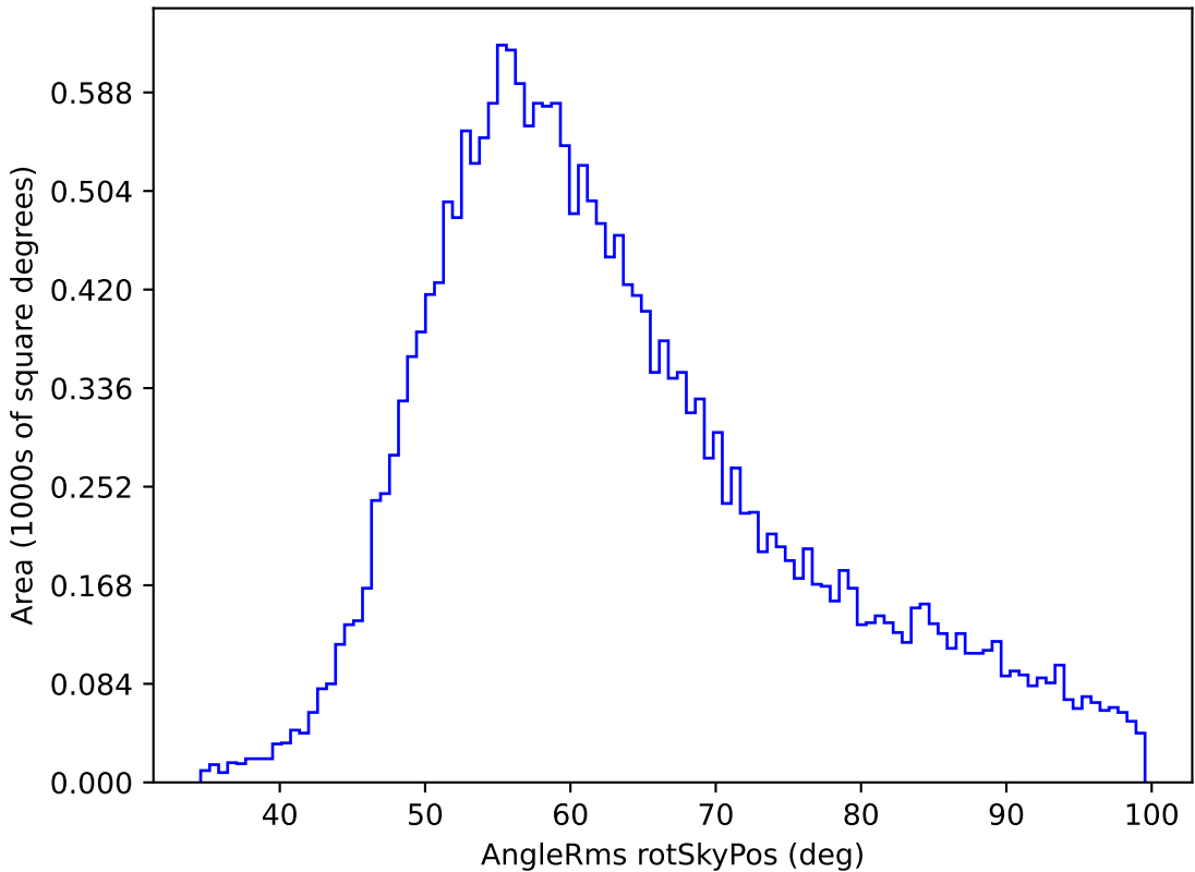
weather_cloudso16v3.4_10yrs All sky u band: AngleRms rotSkyPos
