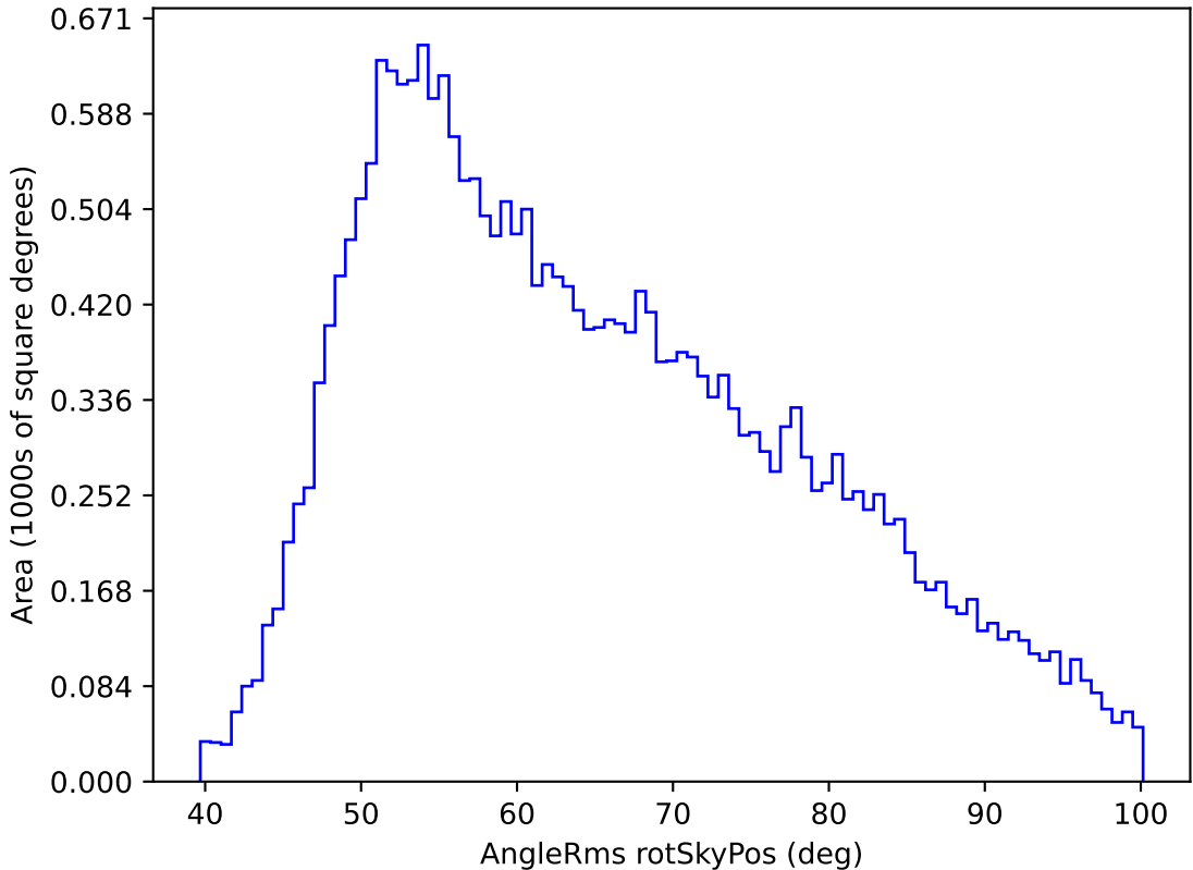
weather_cloudso16v3.4_10yrs All sky g band: AngleRms rotSkyPos
