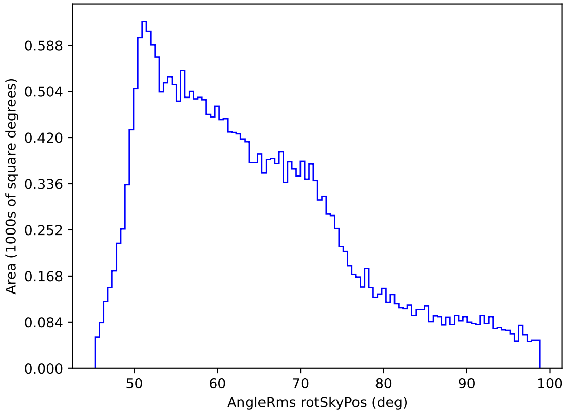
weather_cloudso16v3.4_10yrs All sky all bands: AngleRms rotSkyPos
