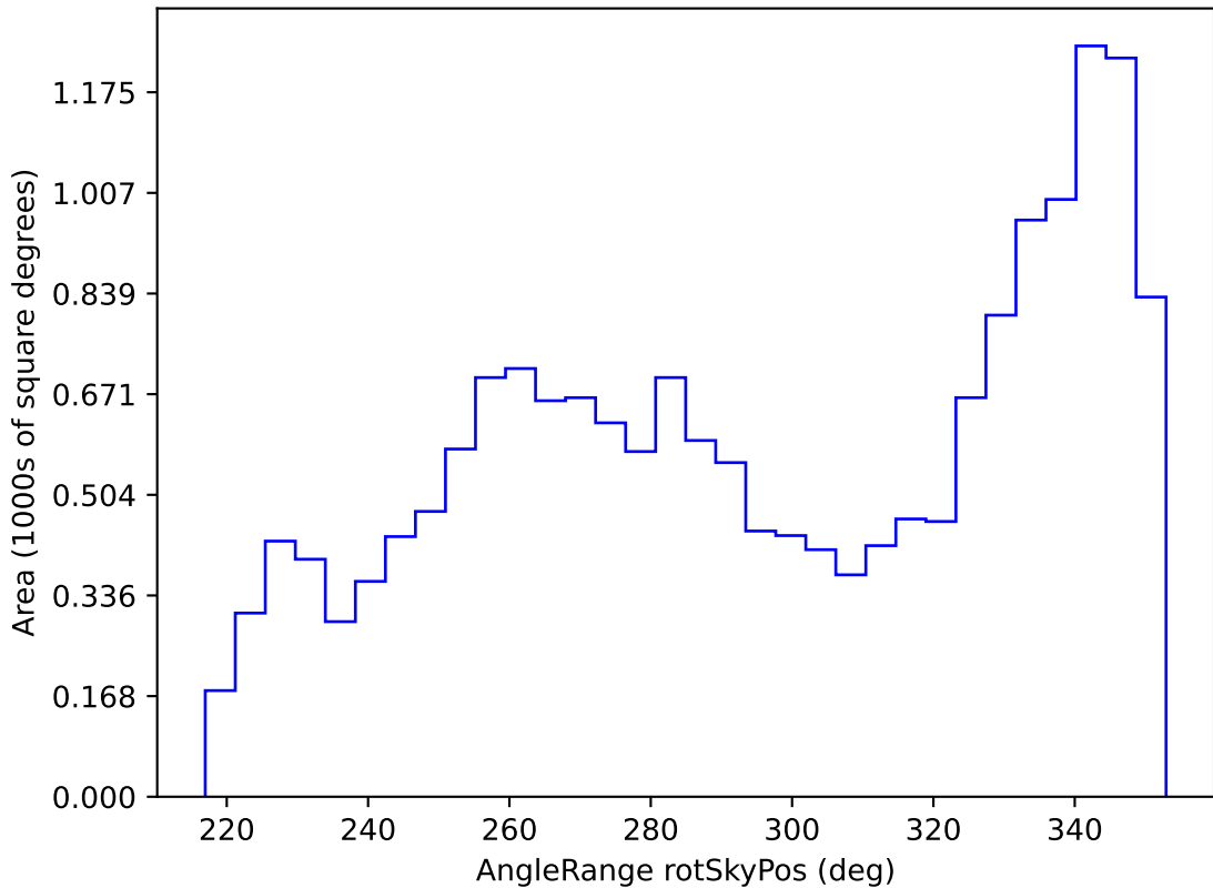
weather_cloudso16v3.4_10yrs WFD all bands: AngleRange rotSkyPos
