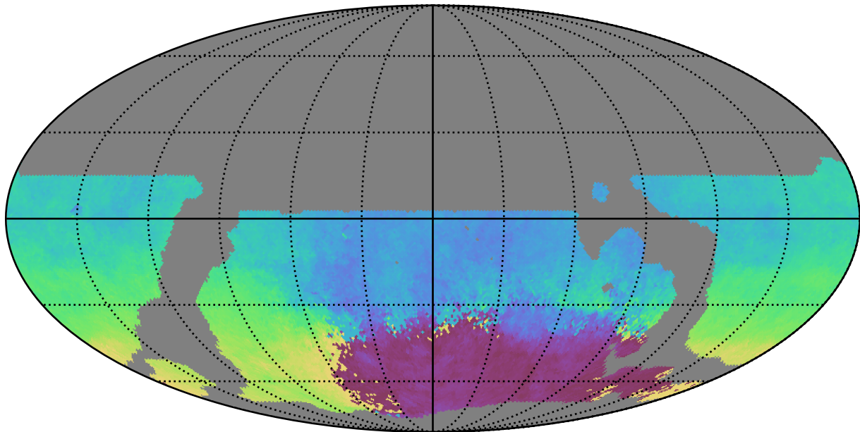
weather_cloudso16v3.4_10yrs WFD u band: AngleMean rotSkyPos
