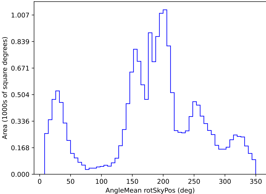
weather_cloudso16v3.4_10yrs WFD u band: AngleMean rotSkyPos
