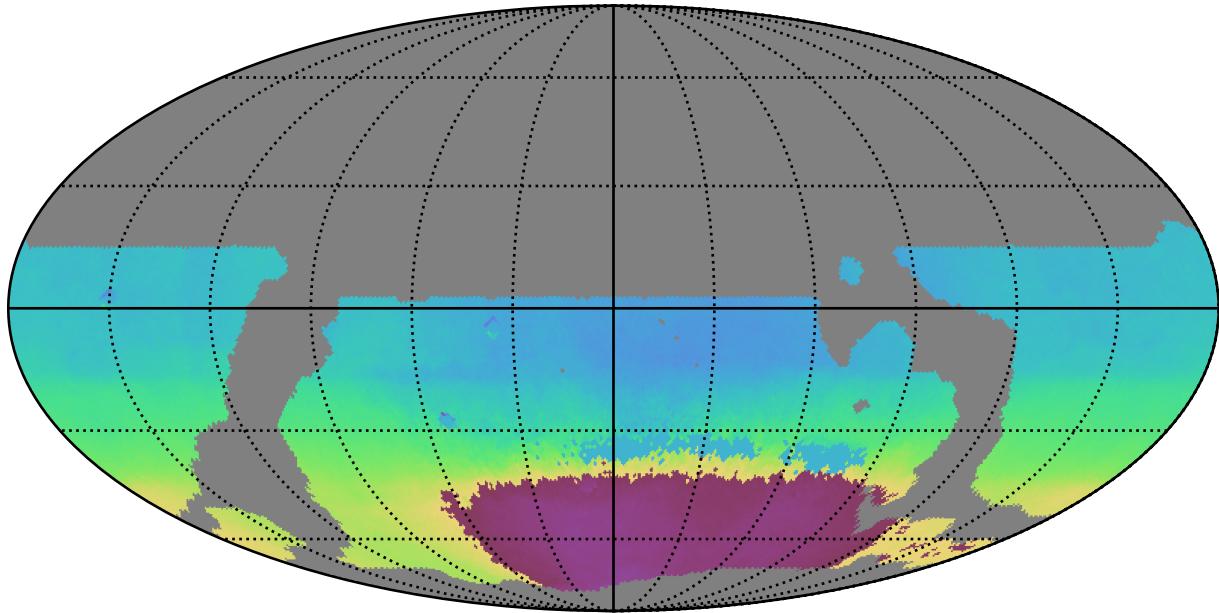
weather_cloudso16v3.4_10yrs WFD all bands: AngleMean rotSkyPos
