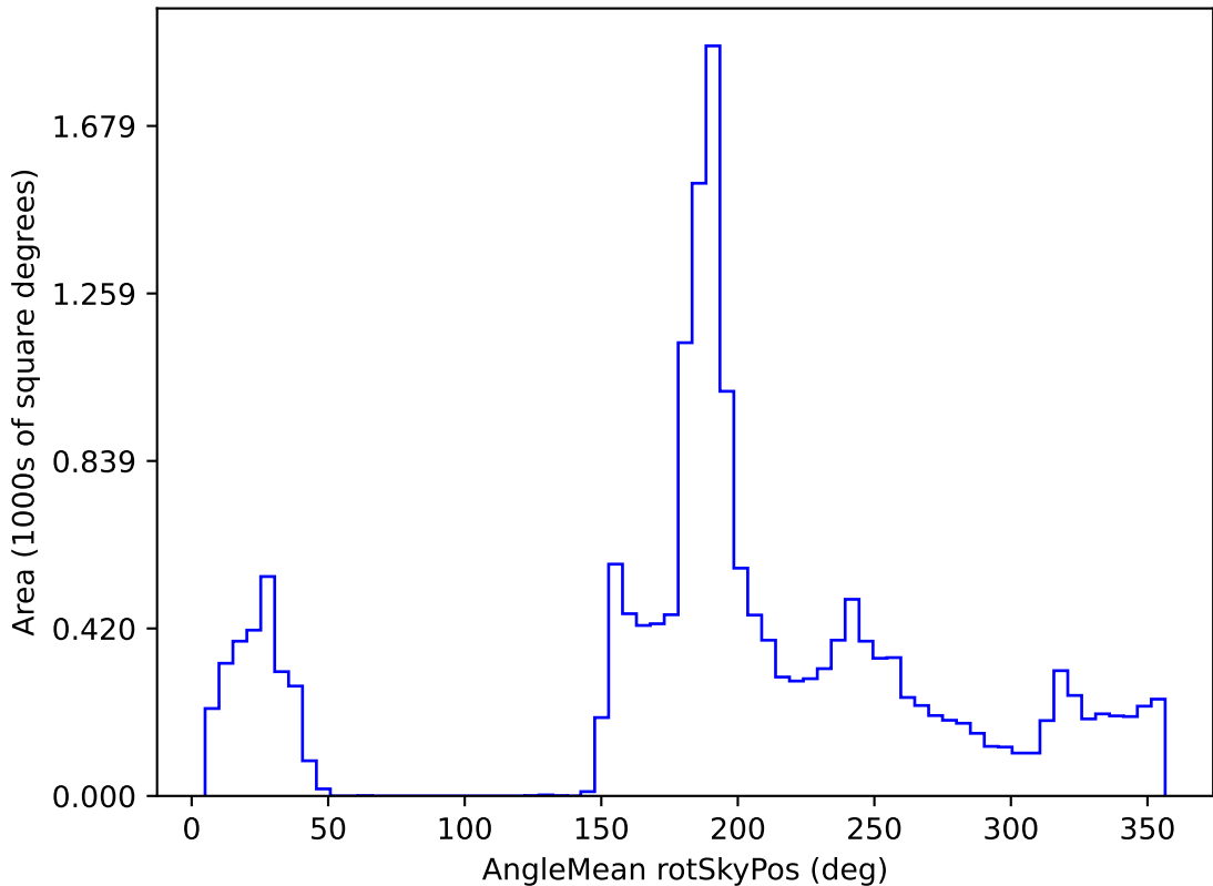
weather_cloudso16v3.4_10yrs WFD all bands: AngleMean rotSkyPos
