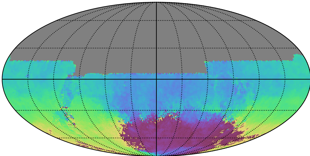
weather_cloudso16v3.4_10yrs All sky u band: AngleMean rotSkyPos
