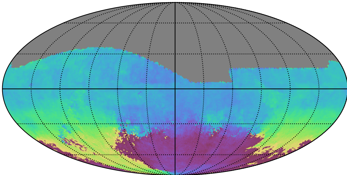
weather_cloudso16v3.4_10yrs All sky g band: AngleMean rotSkyPos
