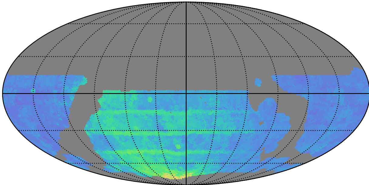
weather_cloudso16v3.4_10yrs WFD z band: 80thPercentile Season Length
