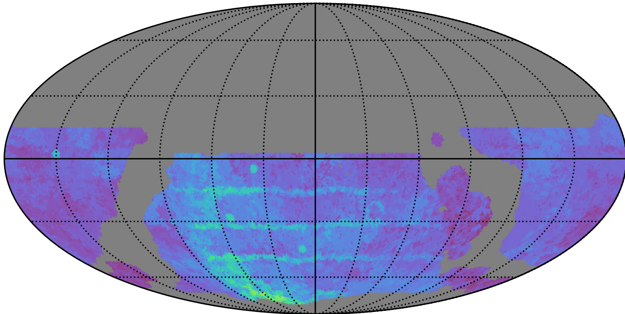
weather_cloudso16v3.4_10yrs WFD u band: 80thPercentile Season Length
