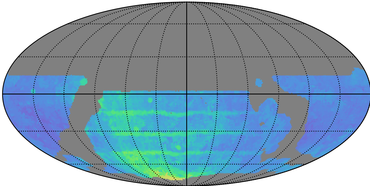
weather_cloudso16v3.4_10yrs WFD r band: 80thPercentile Season Length
