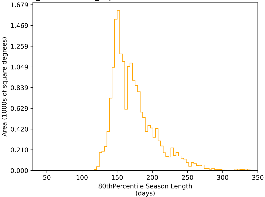
weather_cloudso16v3.4_10yrs WFD r band: 80thPercentile Season Length
