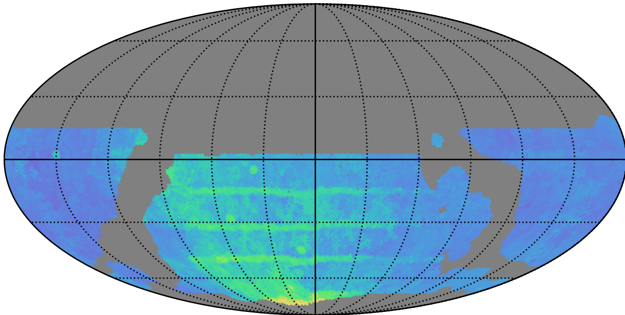
weather_cloudso16v3.4_10yrs WFD i band: 80thPercentile Season Length
