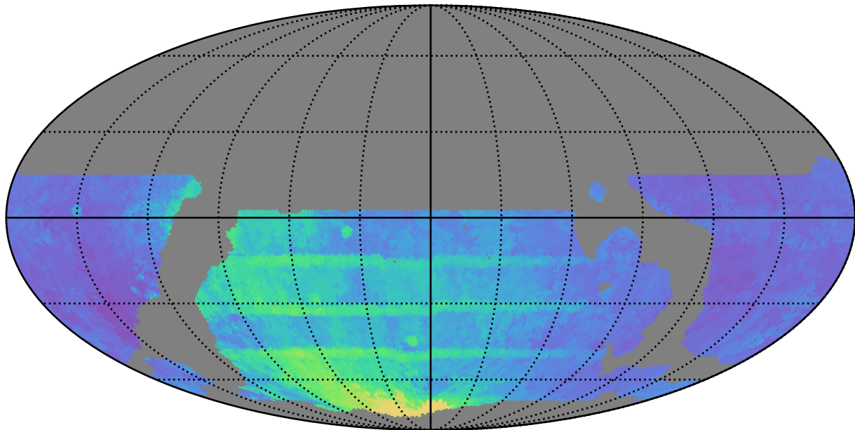
weather_cloudso16v3.4_10yrs WFD all bands: 80thPercentile Season Length
