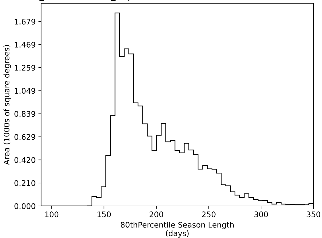
weather_cloudso16v3.4_10yrs WFD all bands: 80thPercentile Season Length
