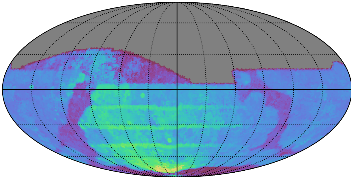
weather_cloudso16v3.4_10yrs All sky z band: 80thPercentile Season Length
