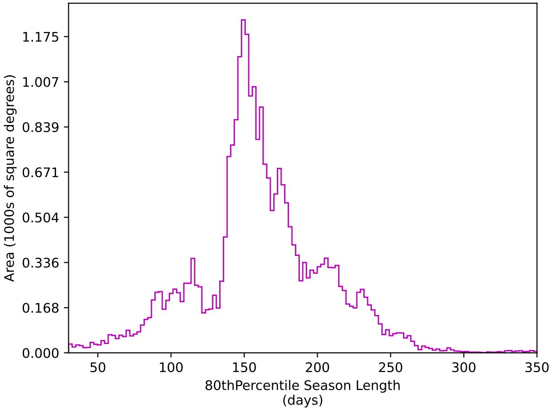
weather_cloudso16v3.4_10yrs All sky z band: 80thPercentile Season Length
