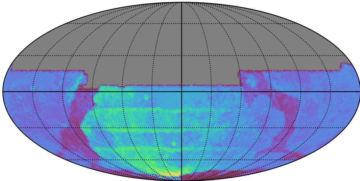
weather_cloudso16v3.4_10yrs All sky y band: 80thPercentile Season Length
