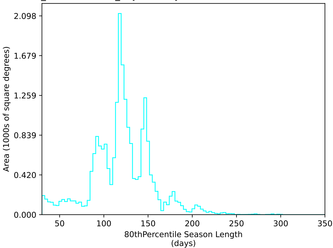
weather_cloudso16v3.4_10yrs All sky u band: 80thPercentile Season Length
