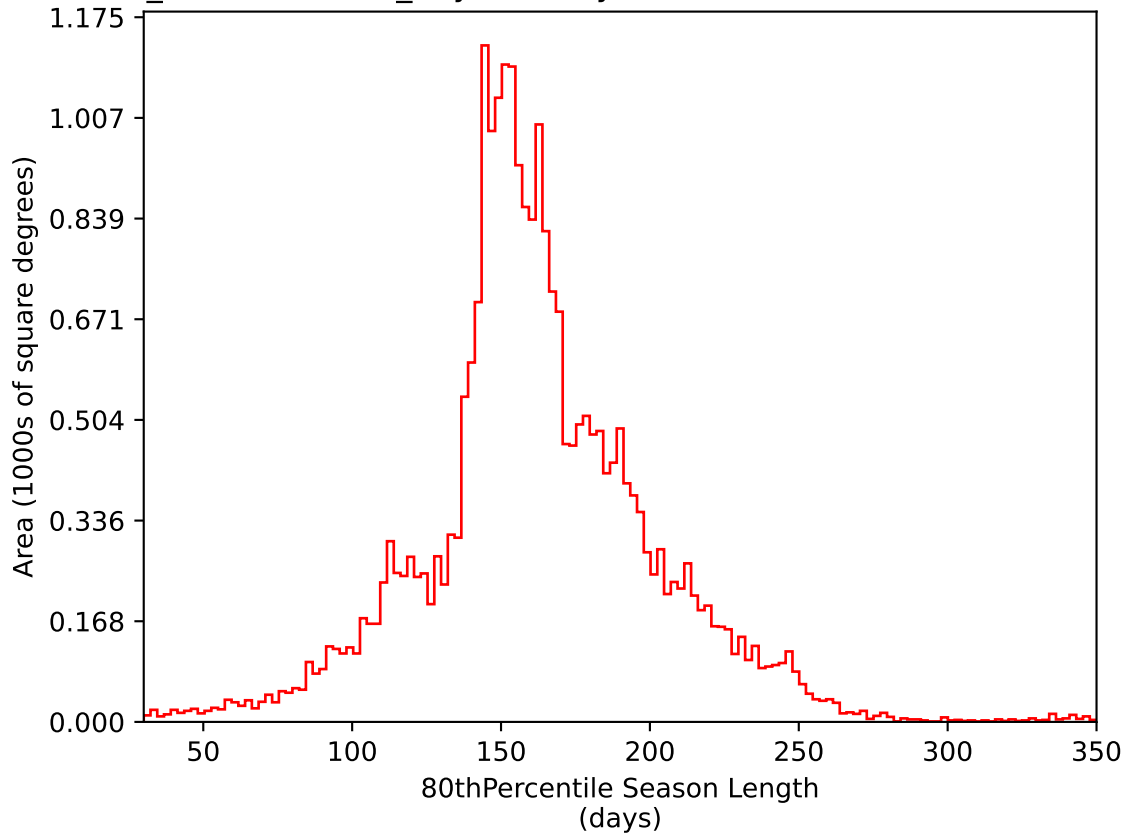
weather_cloudso16v3.4_10yrs All sky i band: 80thPercentile Season Length
