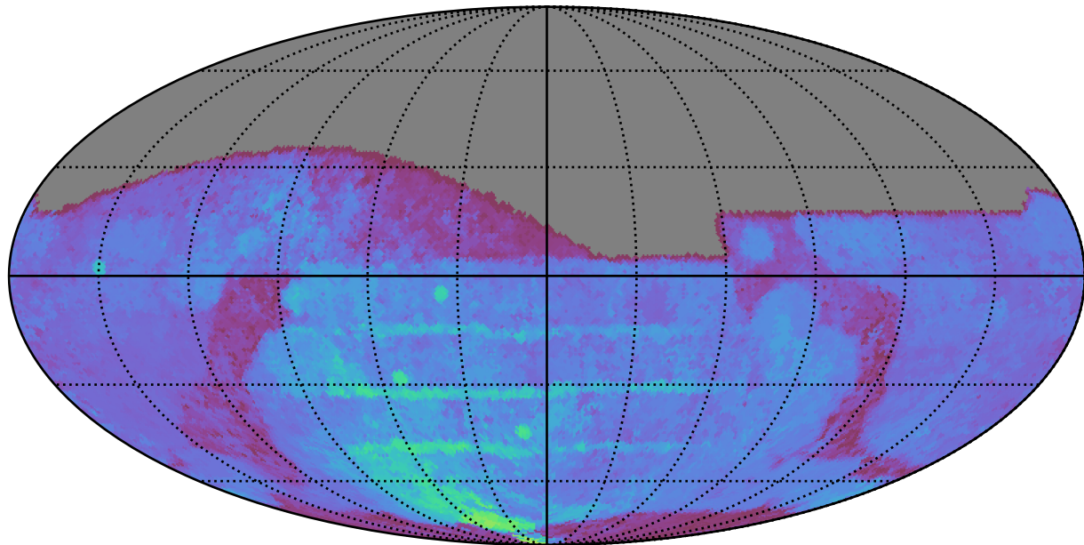
weather_cloudso16v3.4_10yrs All sky g band: 80thPercentile Season Length
