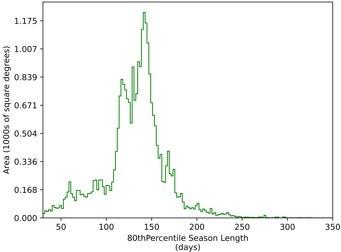
weather_cloudso16v3.4_10yrs All sky g band: 80thPercentile Season Length
