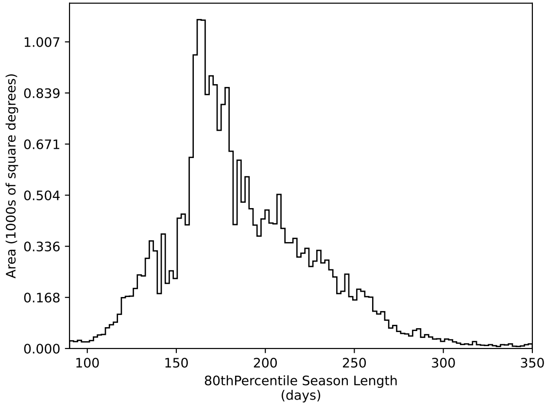
weather_cloudso16v3.4_10yrs All sky all bands: 80thPercentile Season Length
