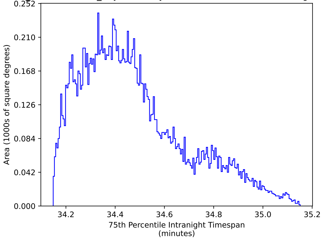
weather_cloudso16v3.4_10yrs WFD zy bands: 75th Percentile Intranight Timespan
