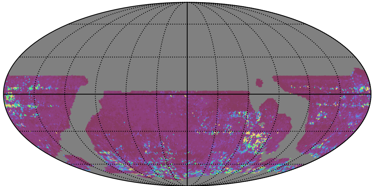
weather_cloudso16v3.4_10yrs WFD z band: 75th Percentile Intranight Timespan
