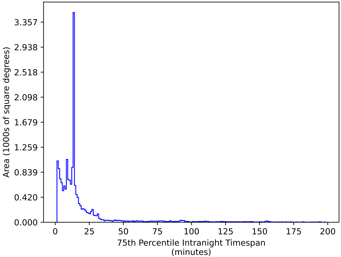
weather_cloudso16v3.4_10yrs WFD z band: 75th Percentile Intranight Timespan
