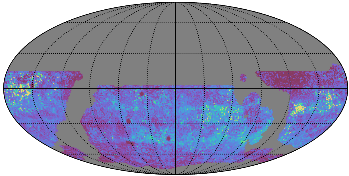
weather_cloudso16v3.4_10yrs WFD y band: 75th Percentile Intranight Timespan
