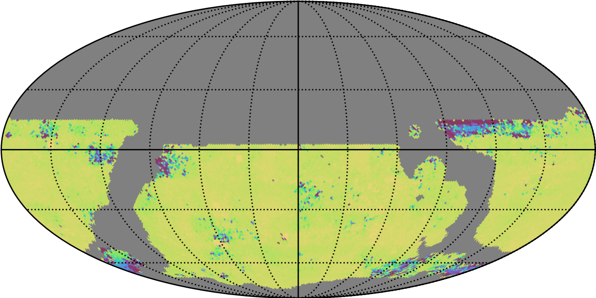
weather_cloudso16v3.4_10yrs WFD ug bands: 75th Percentile Intranight Timespan
