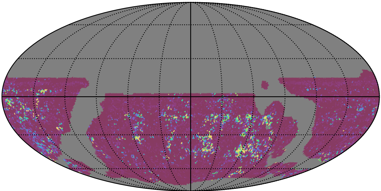
weather_cloudso16v3.4_10yrs WFD u band: 75th Percentile Intranight Timespan
