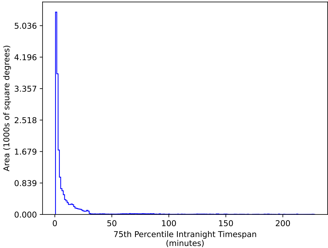
weather_cloudso16v3.4_10yrs WFD u band: 75th Percentile Intranight Timespan
