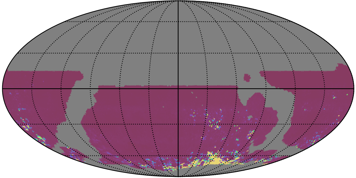
weather_cloudso16v3.4_10yrs WFD ri bands: 75th Percentile Intranight Timespan
