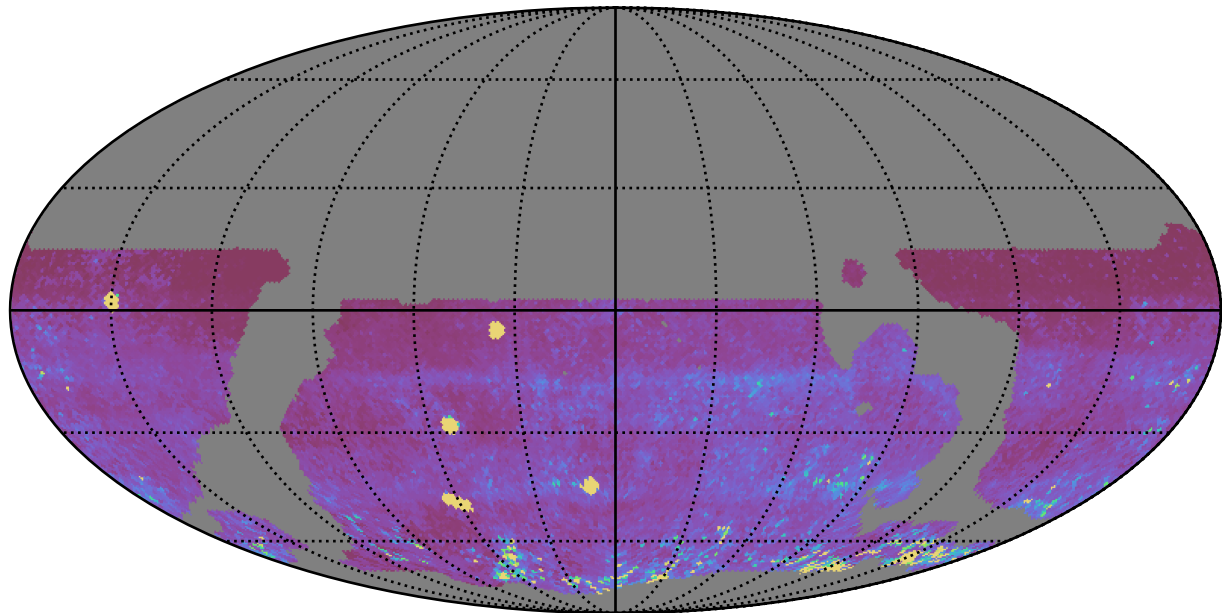
weather_cloudso16v3.4_10yrs WFD iz bands: 75th Percentile Intranight Timespan
