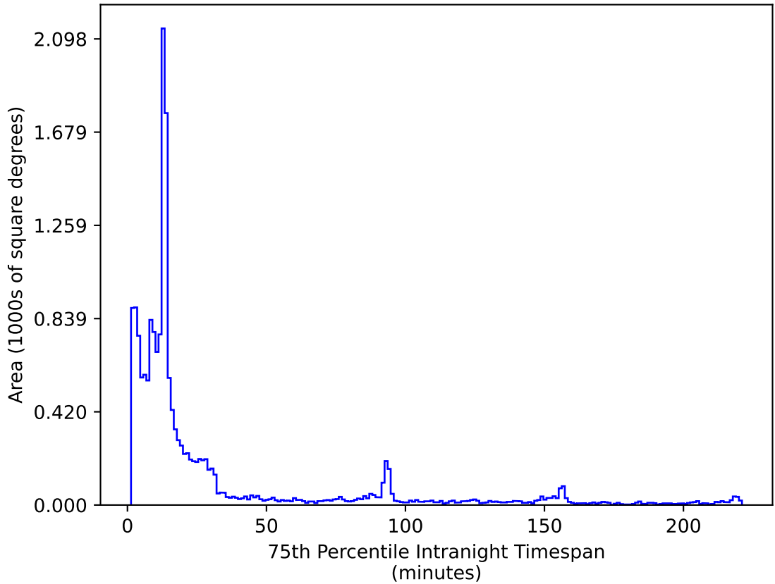
weather_cloudso16v3.4_10yrs WFD i band: 75th Percentile Intranight Timespan
