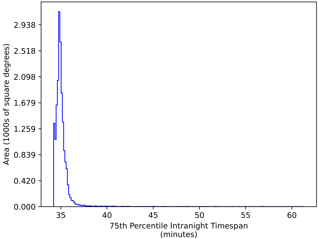
weather_cloudso16v3.4_10yrs WFD gr bands: 75th Percentile Intranight Timespan
