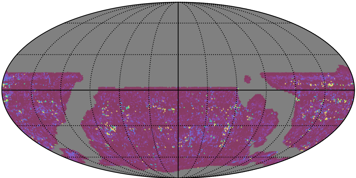
weather_cloudso16v3.4_10yrs WFD g band: 75th Percentile Intranight Timespan
