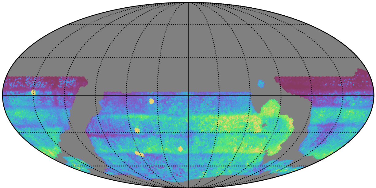
weather_cloudso16v3.4_10yrs WFD all bands: 75th Percentile Intranight Timespan
