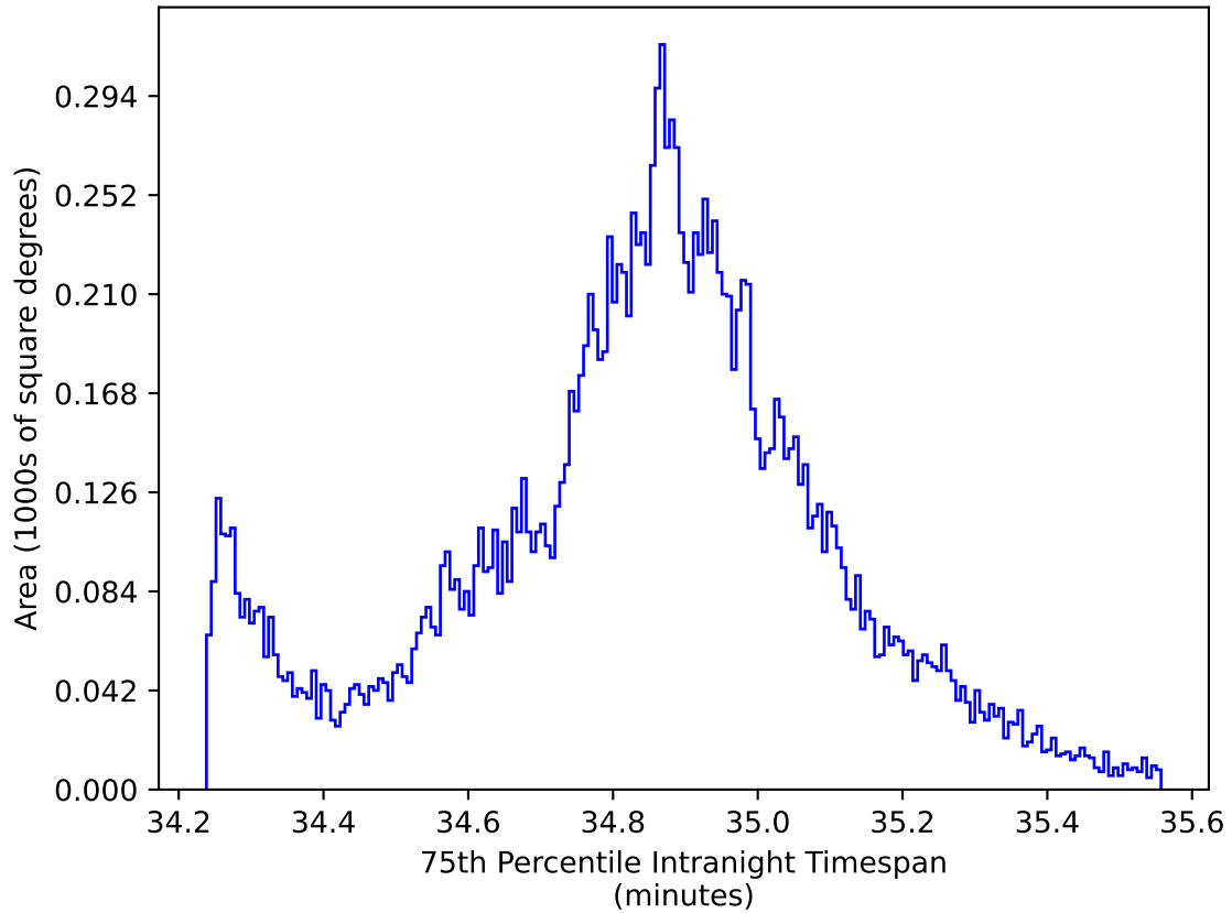
weather_cloudso16v3.4_10yrs WFD all bands: 75th Percentile Intranight Timespan
