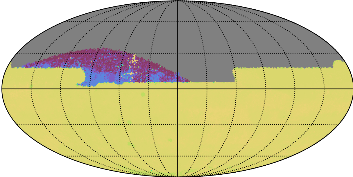
weather_cloudso16v3.4_10yrs All sky zy bands: 75th Percentile Intranight Timespan
